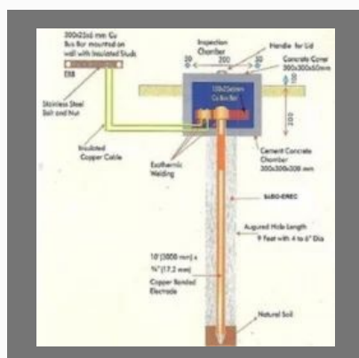
GI Earthing Electrodes
